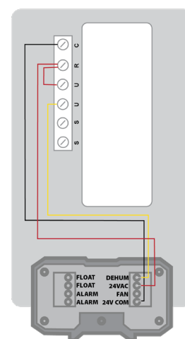
4041649 HONEYWELL HUMIDIPRO WIRING DIAGRAM
