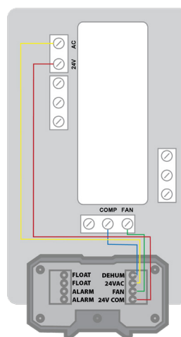
4028531 QUEST DEH 3000R CONTROL WIRING DIAGRAM
