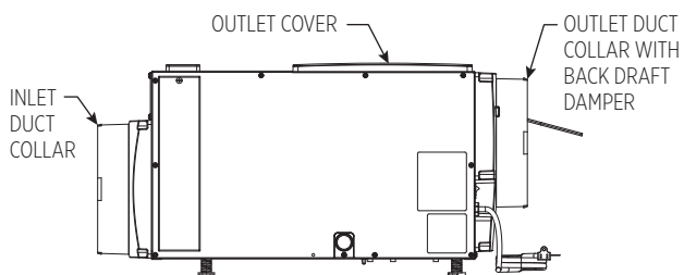
FIGURE 3 – HANGING INSTALL WITH DUCTING
