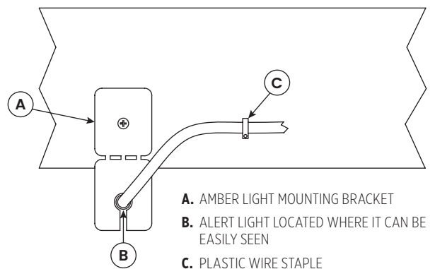
FIGURE 9: ALERT LIGHT MOUNTING
