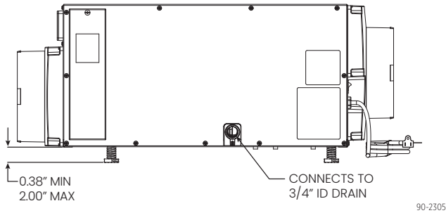
FIGURE 7: LEVELING THE UNIT
