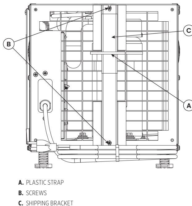
FIGURE 1: PREPARING THE UNIT FOR INSTALLATION
