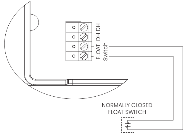
FIGURE 8: FLOAT SWITCH WIRING
