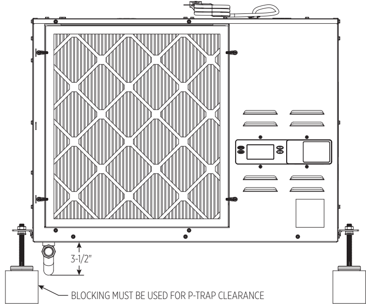
FIGURE 4 - FLOOR MOUNTING
