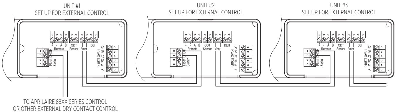
FIGURE 14 – WIRING WITH ALTERNATE EXTERNAL CONTROL
