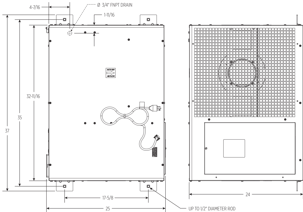
FIGURE 1 – DIMENSIONS (INCHES)
