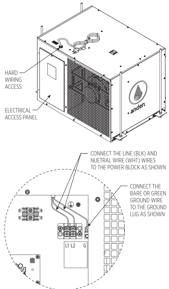
FIGURE 10 – HARD WIRING
