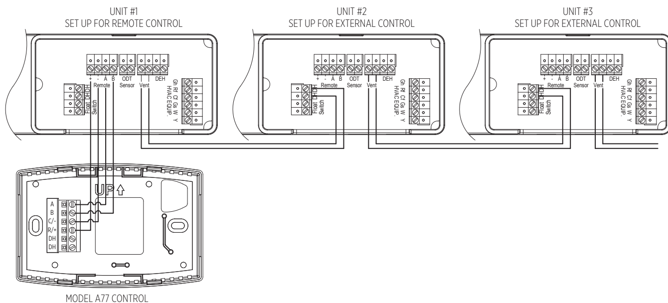
FIGURE 13 – WIRING WITH A77 CONTROL
