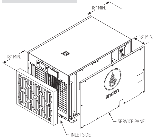
FIGURE 3 – SPACE CLEARANCES
