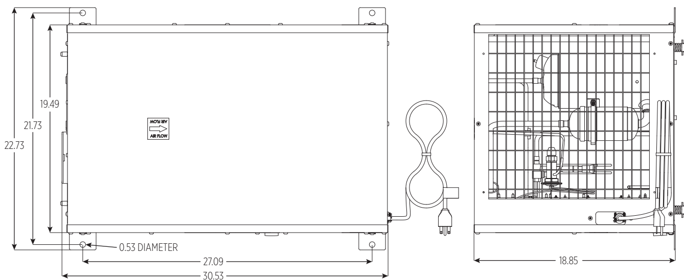
FIGURE 1 – DIMENSIONS (INCHES)
