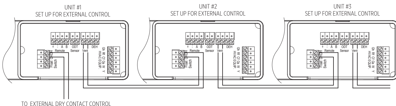
FIGURE 13 – WIRING WITH ALTERNATE EXTERNAL CONTROL
