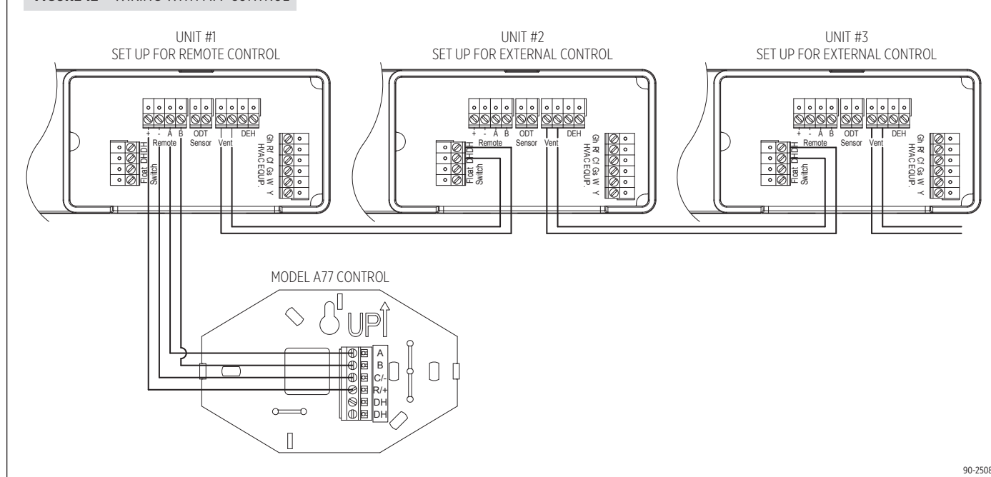
FIGURE 12 – WIRING WITH A77 CONTROL
