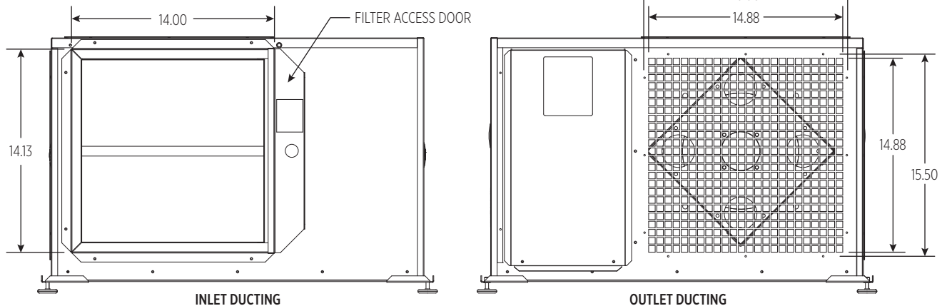
FIGURE 4 – DUCT CONNECTION SIZES (INCHES)
