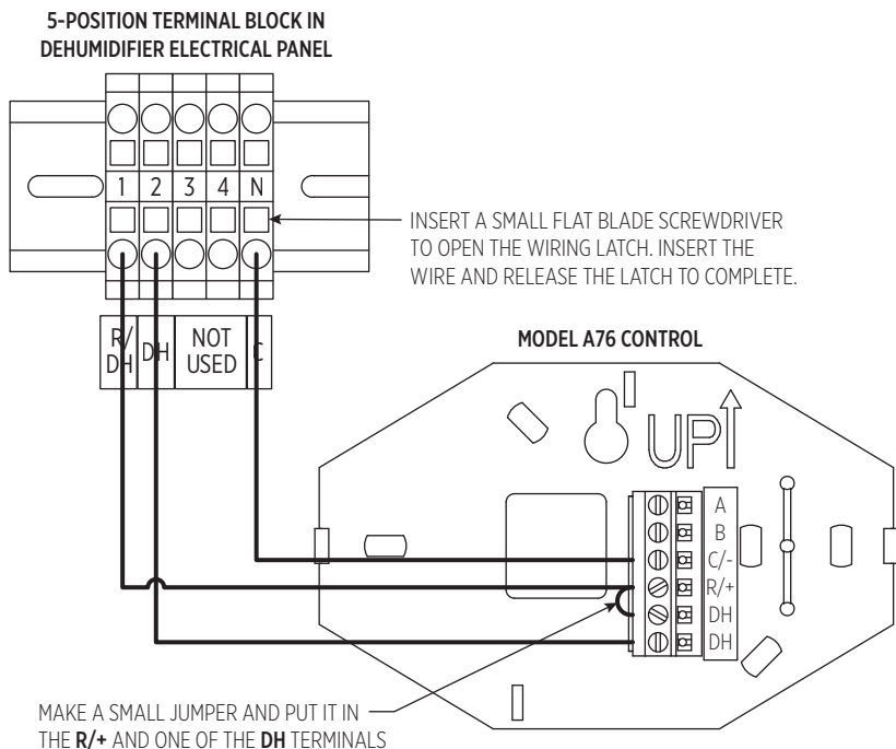
FIGURE 15 – MODEL A76 WIRING
