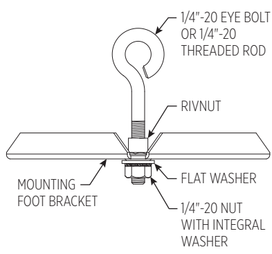
FIGURE 8 – HARDWARE FOR SUSPENDING DEHUMIDIFIER
