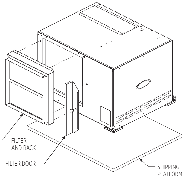
FIGURE 6 – PREPARE UNIT FOR INSTALLATION
