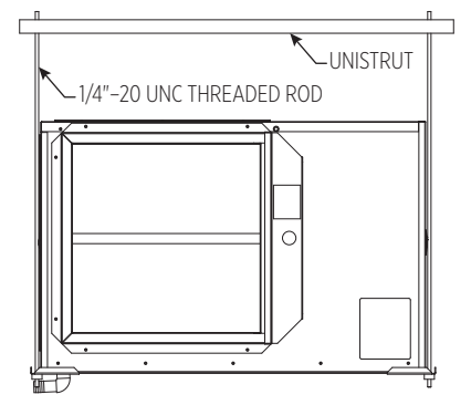
FIGURE 9 – HANGING UNIT WITH THREADED ROD
