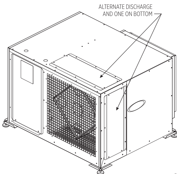
FIGURE 5 – ALTERNATE DISCHARGE LOCATIONS
