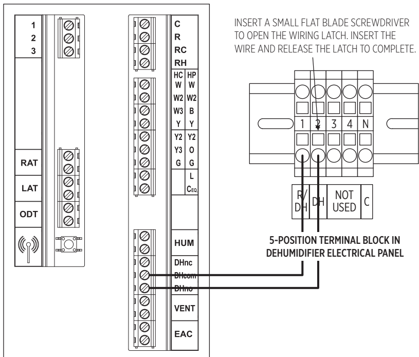
FIGURE 16 – MODEL 8840 WIRING
