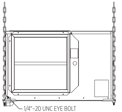
FIGURE 7 – HANGING UNIT WITH CHAIN AND EYE BOLTS
