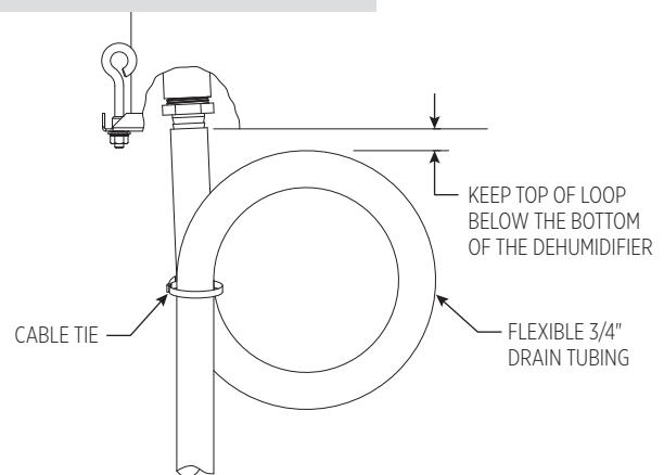
FIGURE 11 – FLEXIBLE DRAIN TUBING
