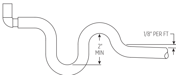
FIGURE 10 – PVC DRAIN TUBING
