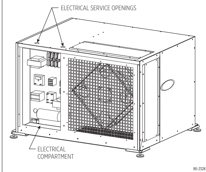
FIGURE 13 – ELECTRICAL CABINET (SERVICE PANEL REMOVED)
