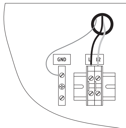
FIGURE 14 – POWER WIRING
