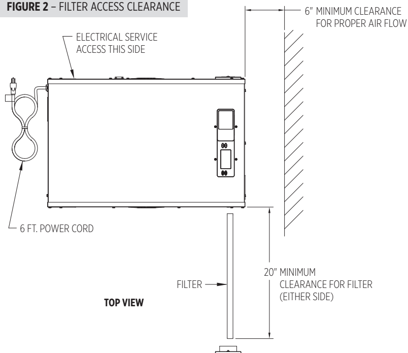
FIGURE 2 – FILTER ACCESS CLEARANCE
