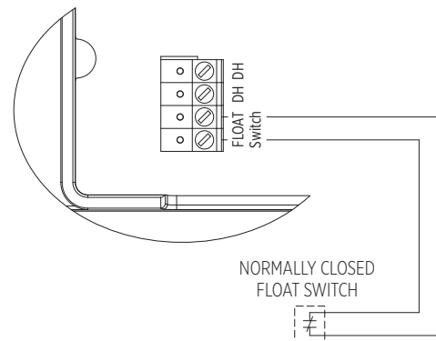
FIGURE 3 – FLOAT SWITCH WIRING
