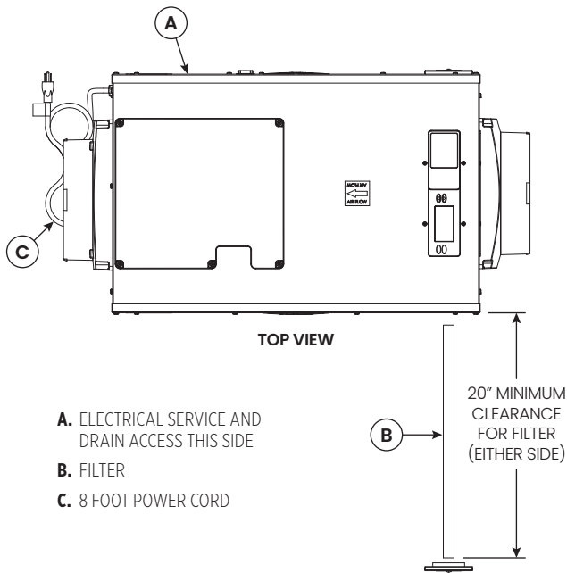
FIGURE 5: FILTER ACCESS CLEARANCE
