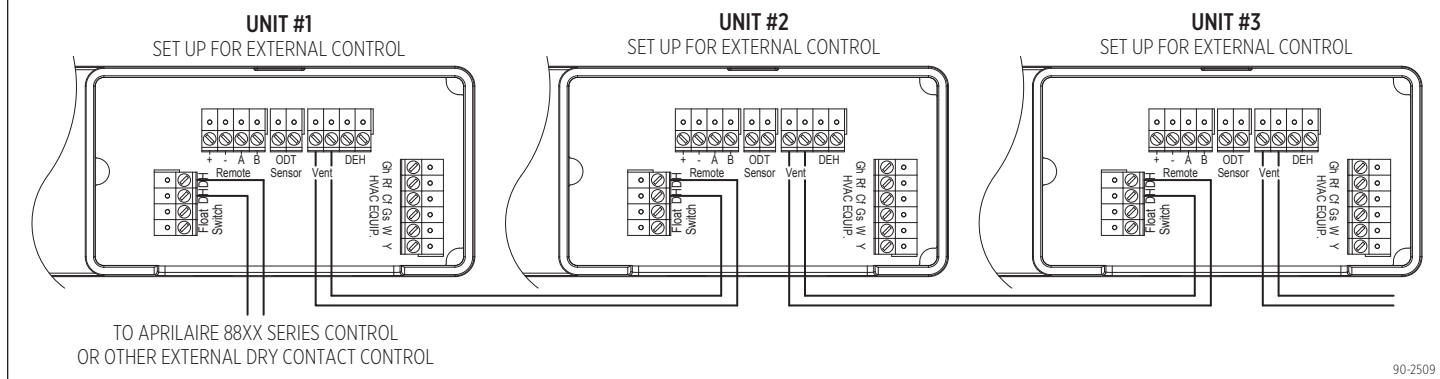
FIGURE 14: DAISY CHAIN WIRING WITH ALTERNATE EXTERNAL CONTROL
