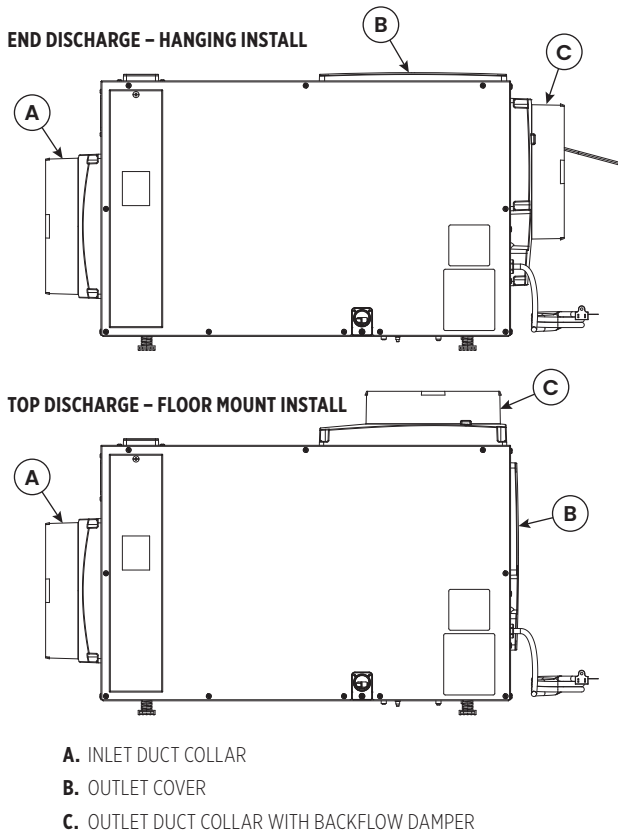
FIGURE 2: FULLY DUCTED INSTALLATIONS
