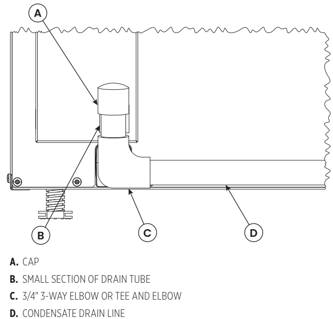
FIGURE 6: CAPPED DRAIN ACCESS FOR CLEANING
