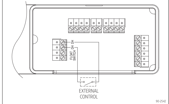
FIGURE 12: ALTERNATIVE EXTERNAL CONTROL WIRING
