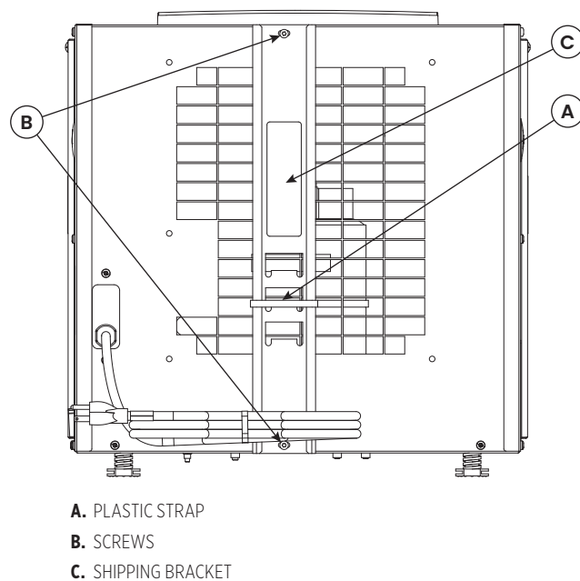
FIGURE 1: PREPARING THE UNIT FOR INSTALLATION
