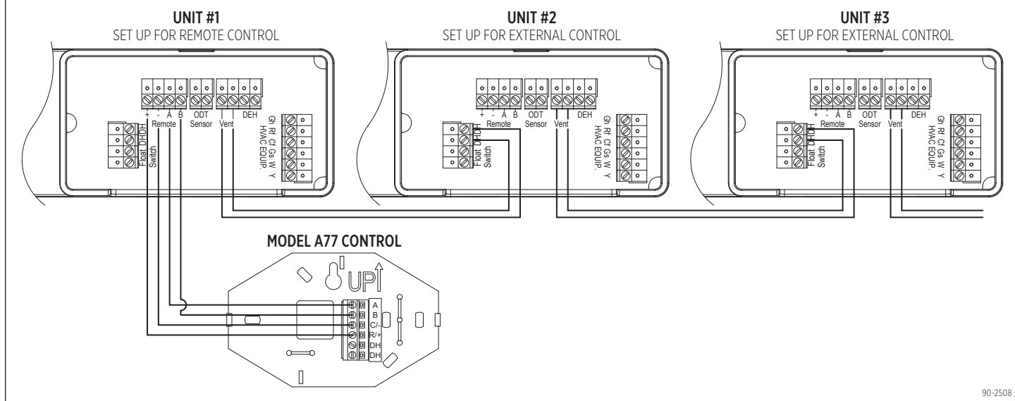
FIGURE 13: DAISY CHAIN WIRING WITH A77 CONTROL
