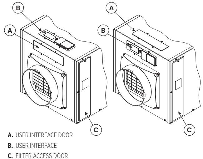
FIGURE 3: USER INTERFACE LOCATION
