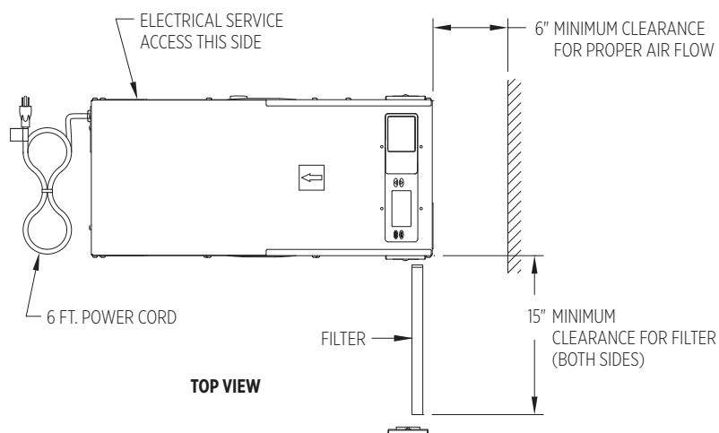
FIGURE 2 – FILTER ACCESS CLEARANCE
