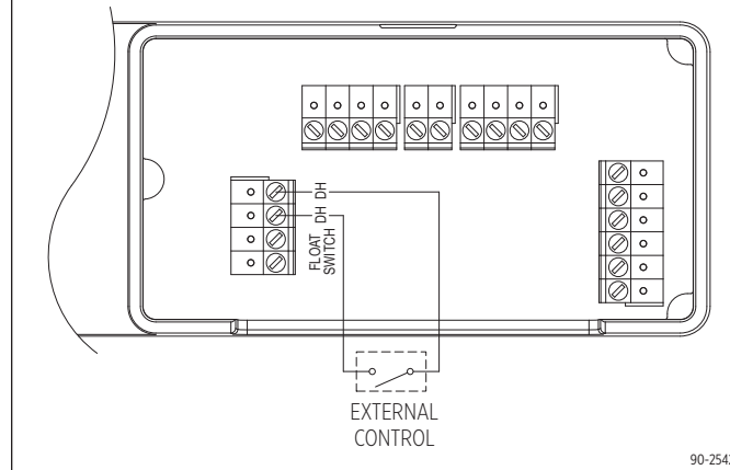
FIGURE 6 – ALTERNATE EXTERNAL CONTROL WIRING
