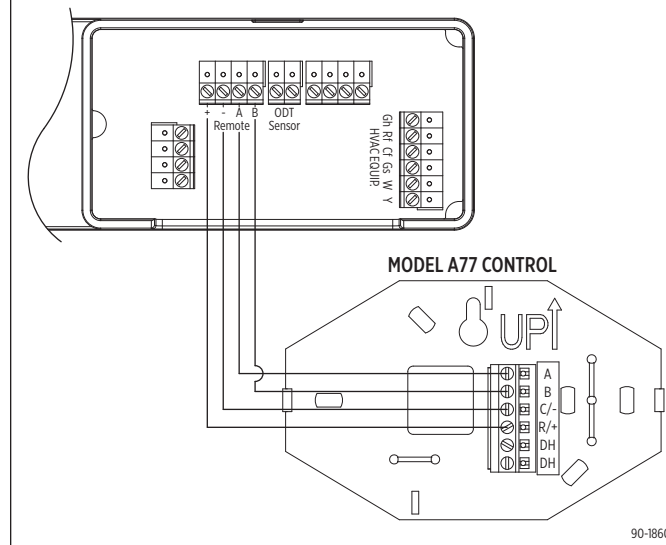
FIGURE 5 – MODEL A77 REMOTE CONTROL WIRING
