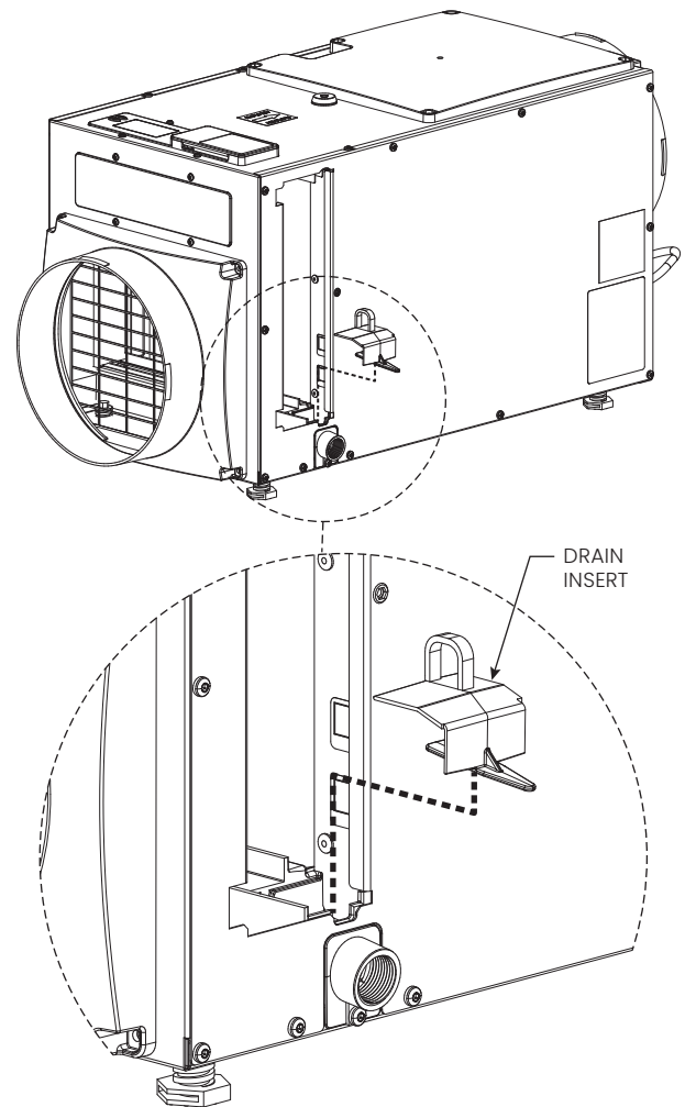
FIGURE 15: DRAIN INSERT
