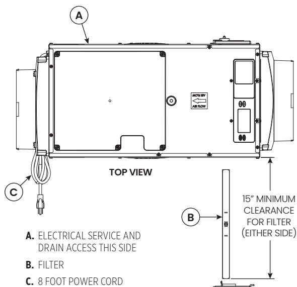
FIGURE 5: FILTER ACCESS CLEARANCE
