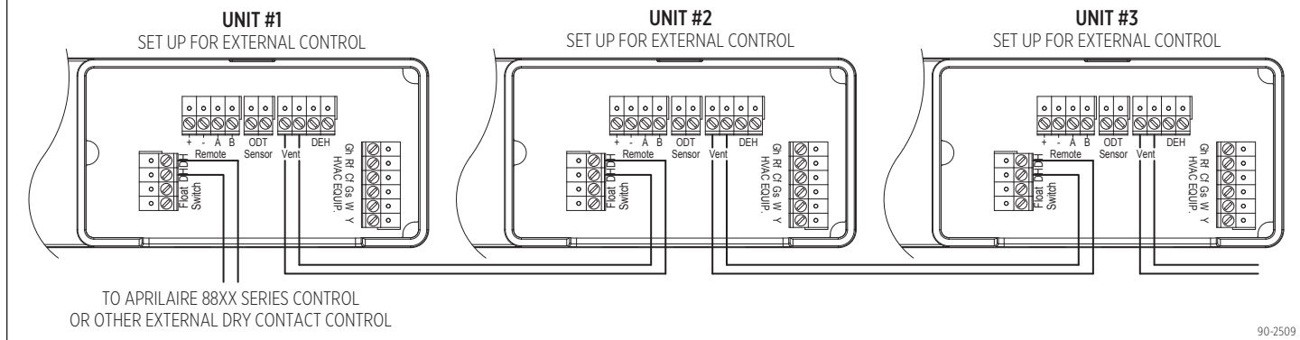
FIGURE 14: DAISY CHAIN WIRING WITH ALTERNATE EXTERNAL CONTROL
