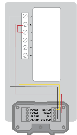
4041649 HONEYWELL HUMIDIPRO WIRING DIAGRAM
